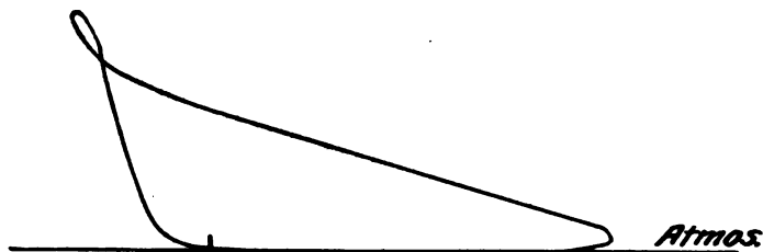
FIG. 50.—Ignition too Early.
